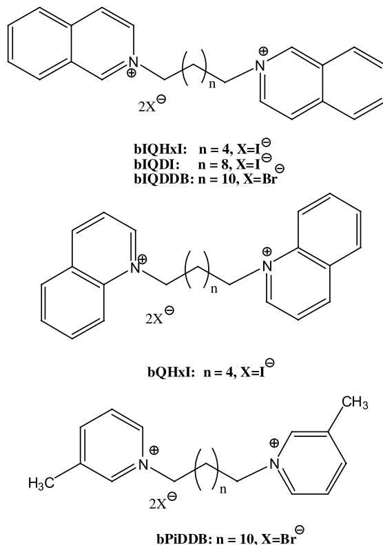
Figure 3. Structures of bis-azaaromatic quaternary ammonium compounds used in this study.
