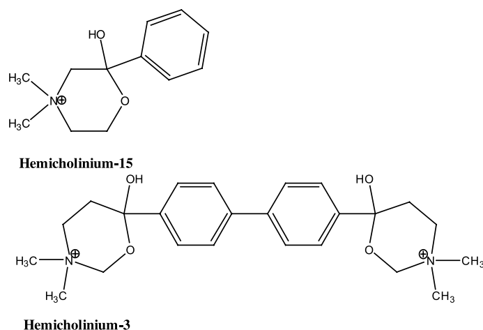
Figure 9. Structures of hemicholinium-3, a bis-quaternary ammonium compound, and its monomer, hemicholinium-15.
