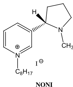
Figure 1. Structure of NONI, a quaternary ammonium compound that has affinity for the BBB-choline transporter. NONI has been shown to be taken up into the brain by the BBB-choline transporter, demonstrating the use of this transporter as a drug delivery vector.
