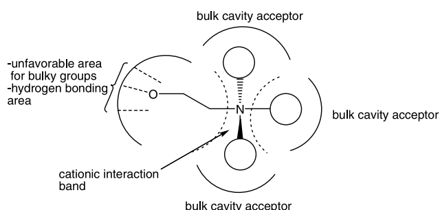
Figure 2. Theoretical rendering of the active binding site of the BBB choline transporter. 2,7,8
